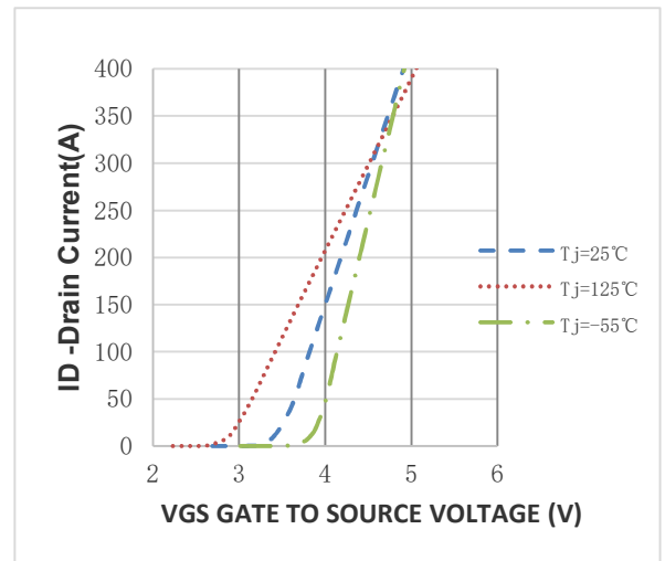
Figure 10. Transfer Characteristics
