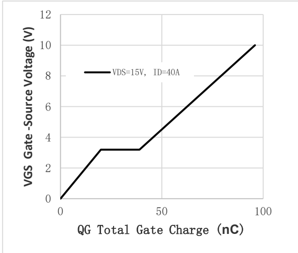
Fig.1 Gate-Charge Characteristics
